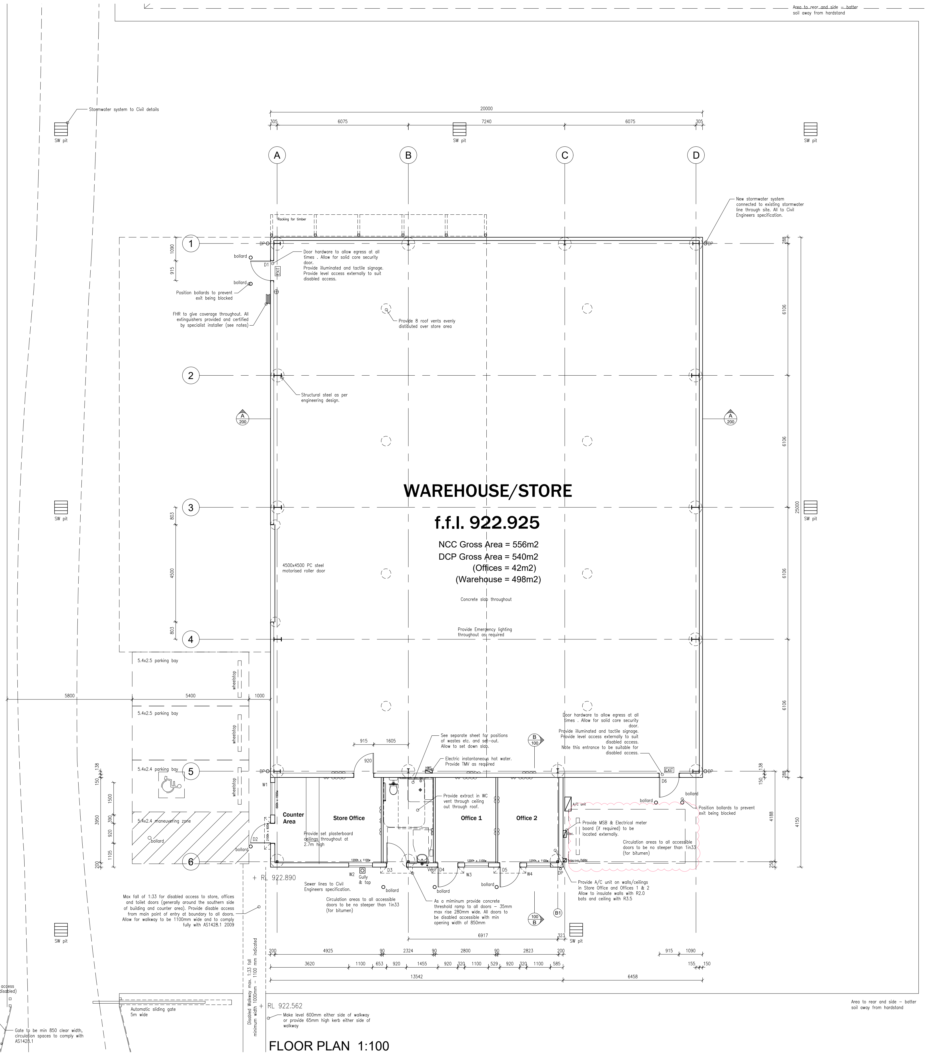
FLOOR PLAN 1:100
